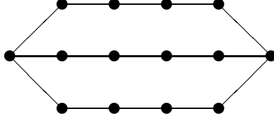
Figure 1: The graph G_1
