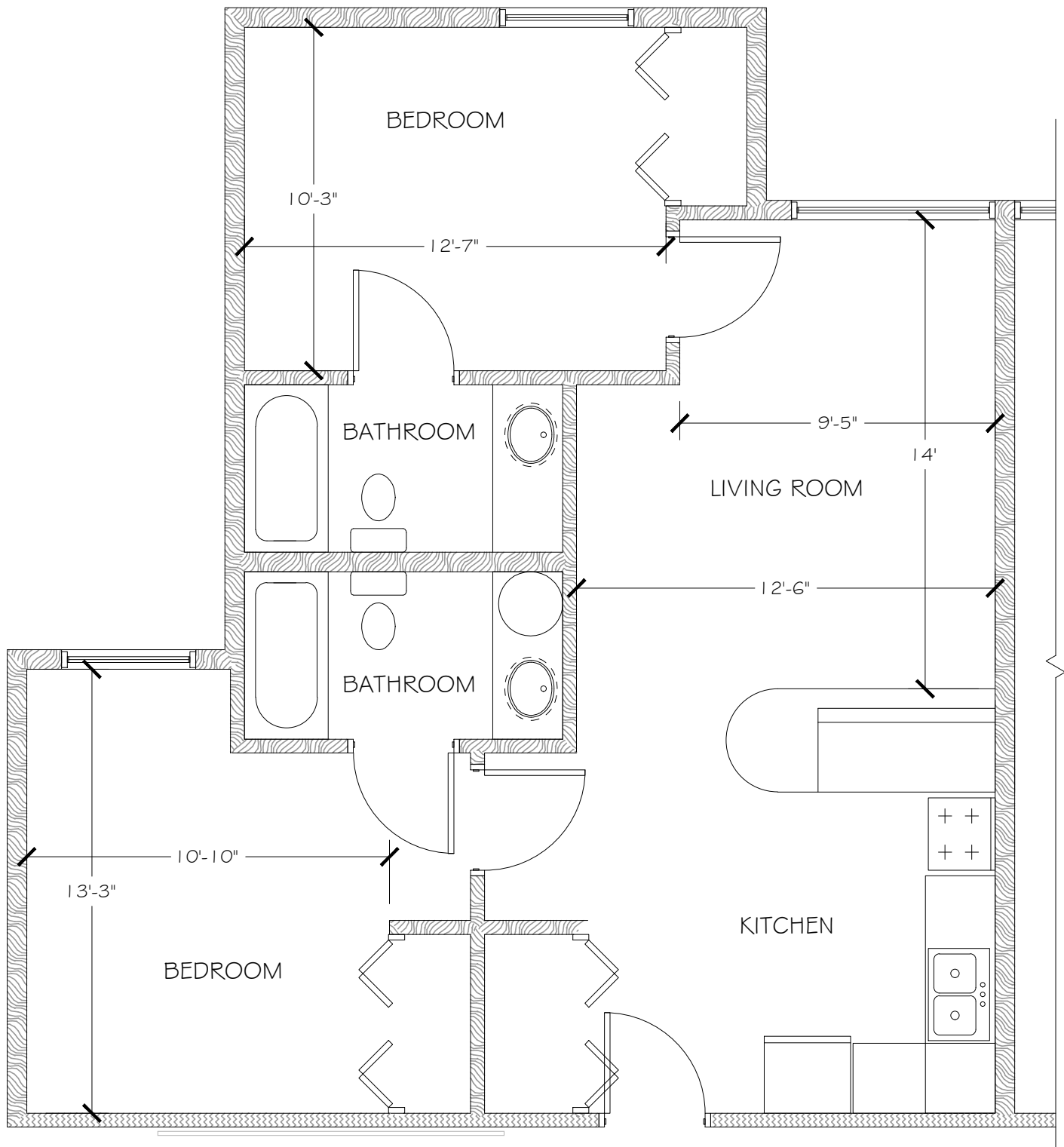
BUC-RIDGE TYP. 2 BEDROOM APARTMENTS P-Q FLOOR PLAN
