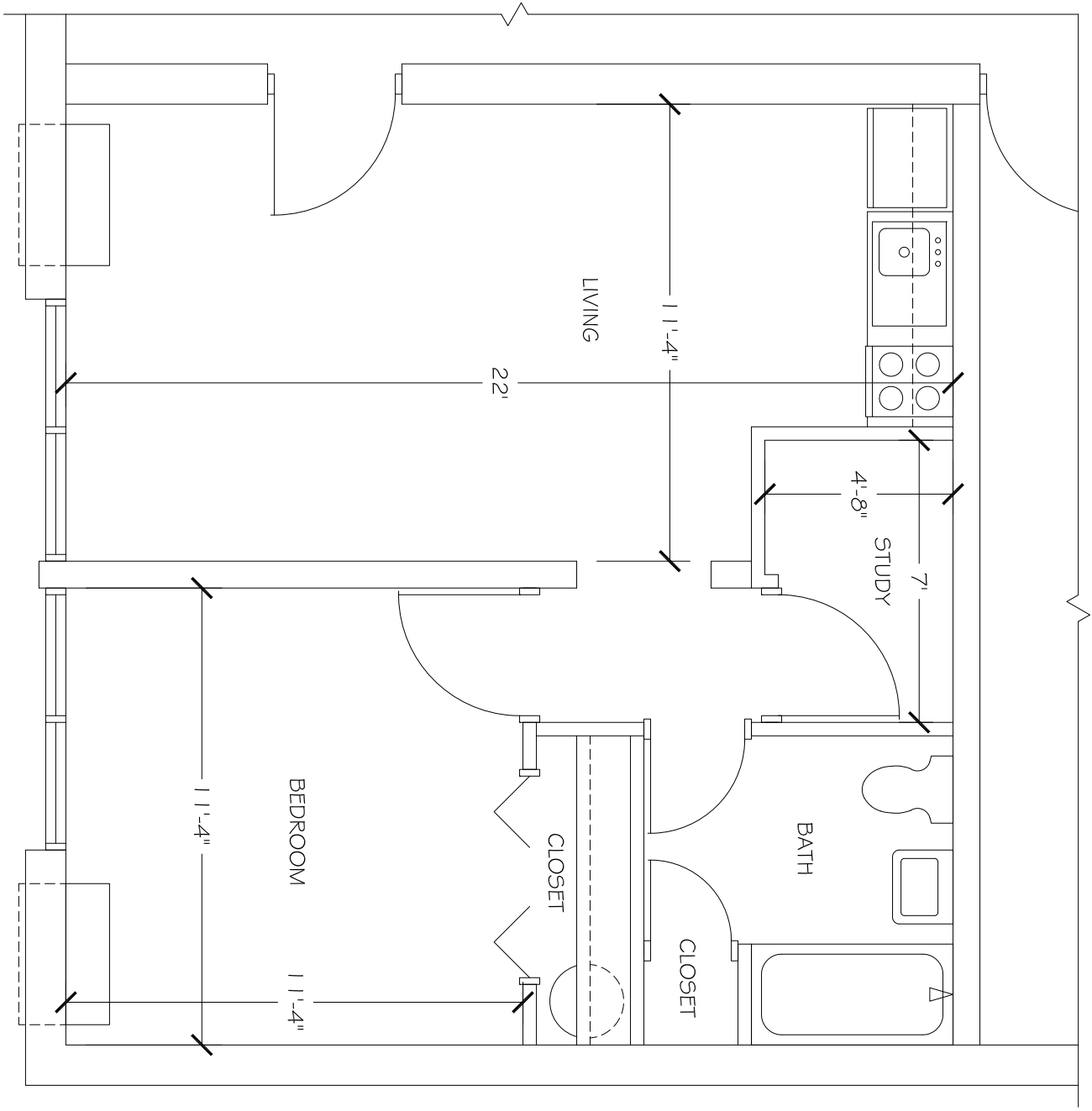
TYP BUC RIDGE BUILDING T-U 1 BEDROOM APARTMENT FLOOR PLAN SCALE: 1/4" = 1'-0"
