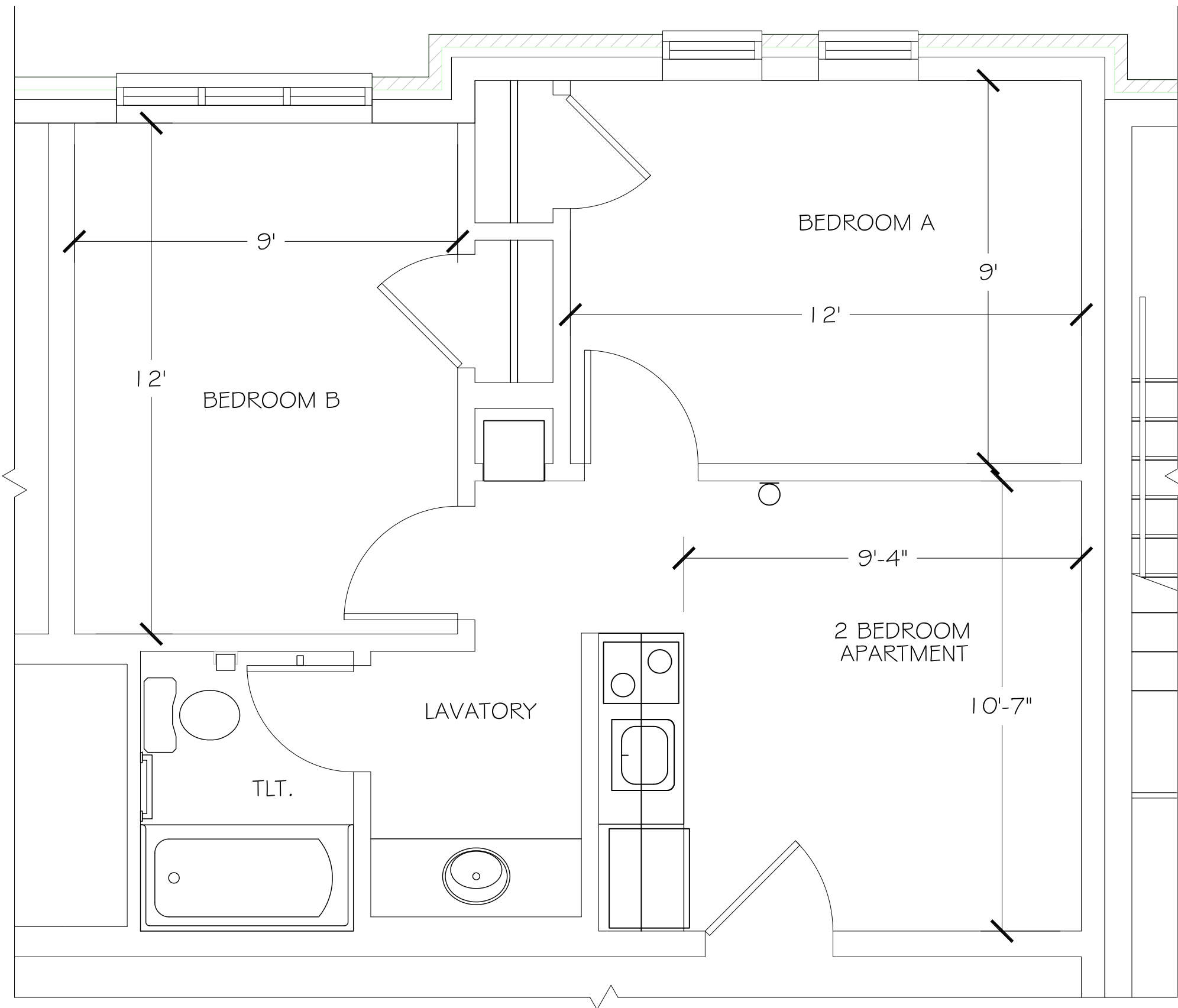
TYP. 2-BEDROOM APARTMENT - FLOOR PLAN SCALE: 3/8" = 1'-0"
