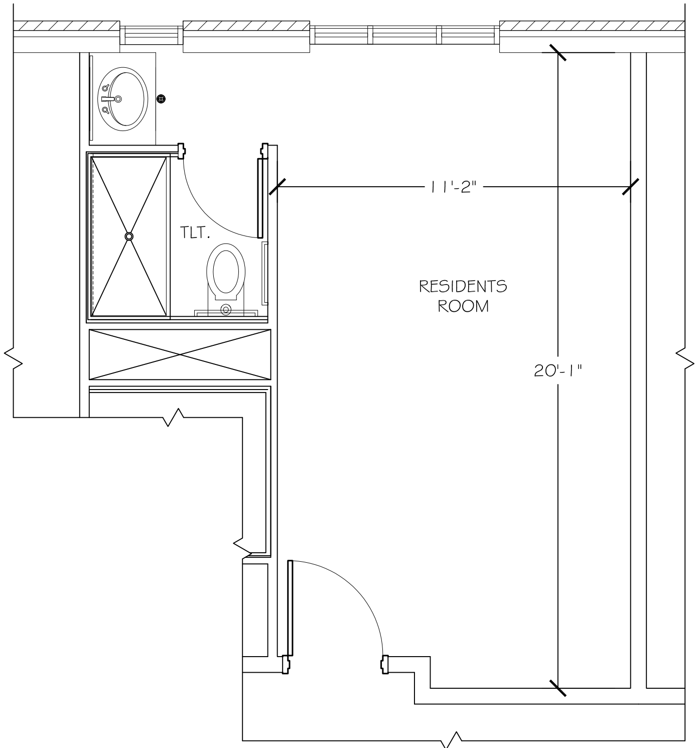
GOVERNORS HALL ROOM LAYOUT
