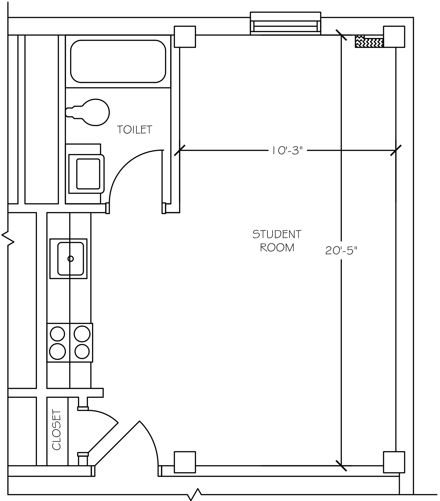
STUDENT ROOM FLOOR PLAN SCALE: 3/8" = 1'-0"
