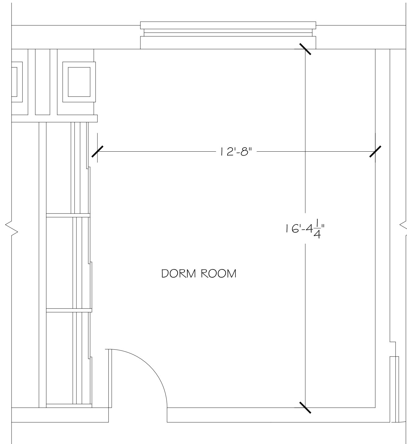
DORM ROOM FLOOR PLAN SCALE: 3/8" = 1'-0"
