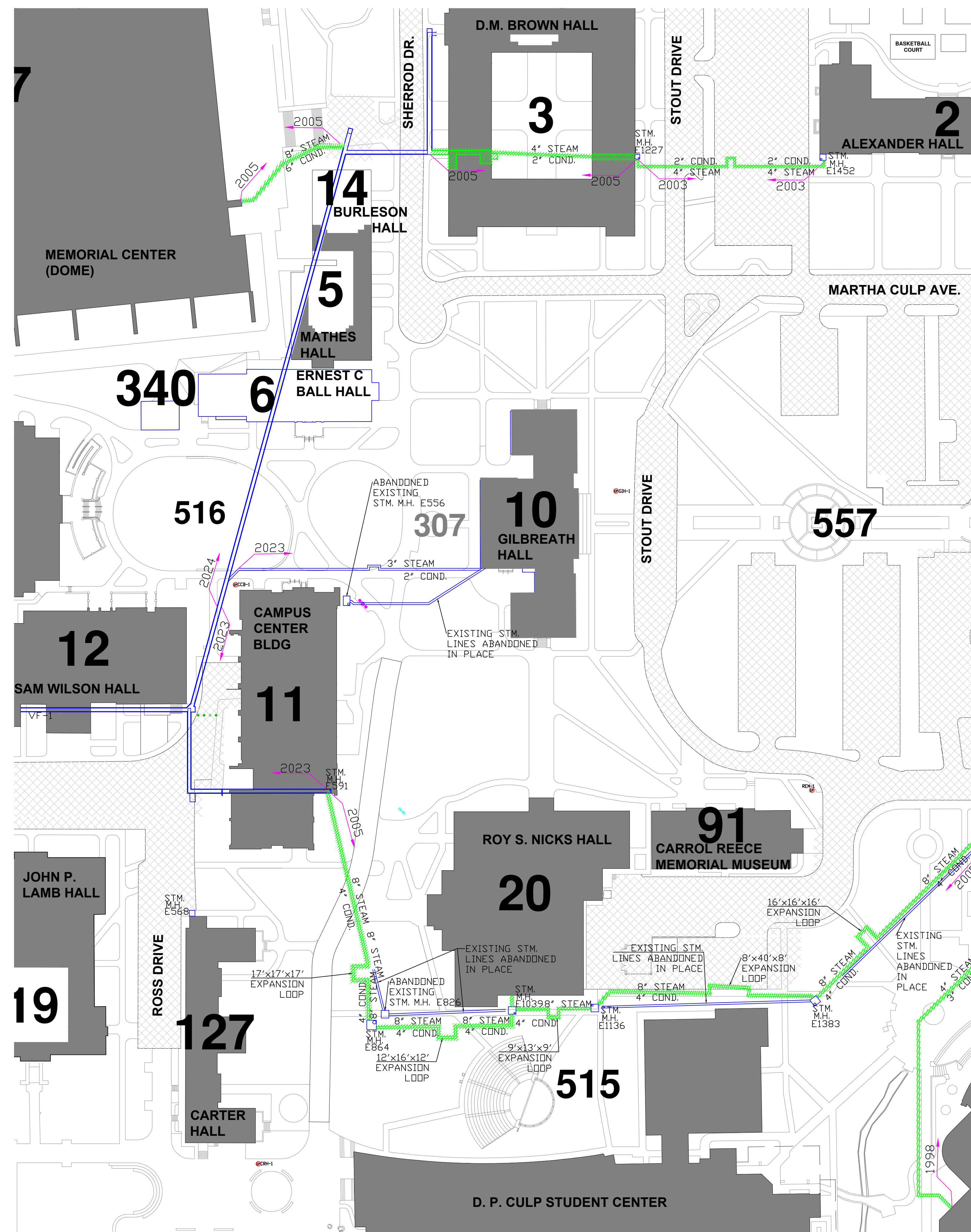
CAMPUS UTILITY REPLACEMENT – MIDDLE EAST SCALE: 1"=60'
