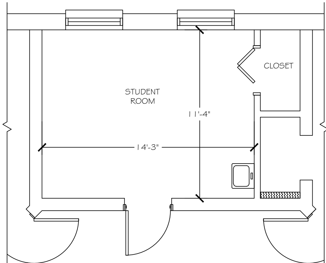
CARTER HALL STUDENT ROOM WITHOUT TOILET FLOOR PLAN
